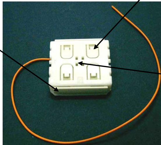
Figure 1: Electro-dynamic powered radio transmitter device PTM 200C
