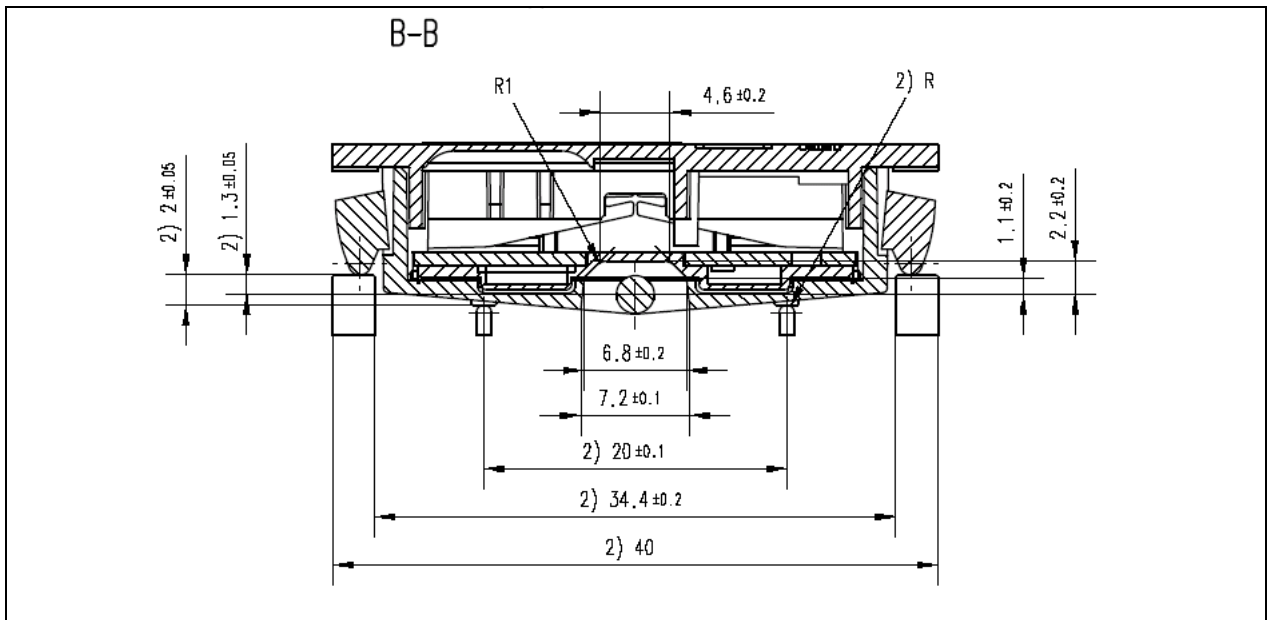
Figure 5: PTM 200C without antenna, cut B and C
