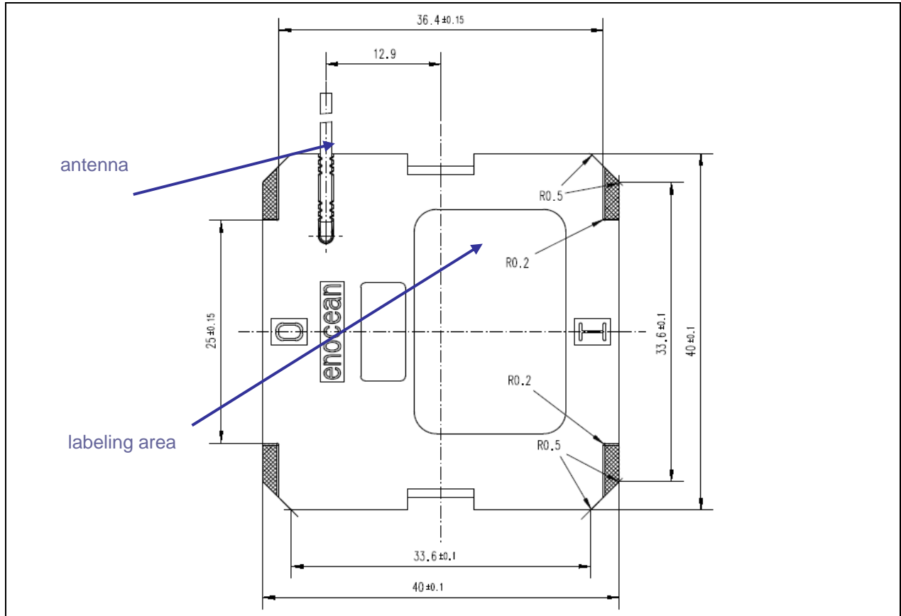
Figure 6: PTM 200C with antenna, rear view
