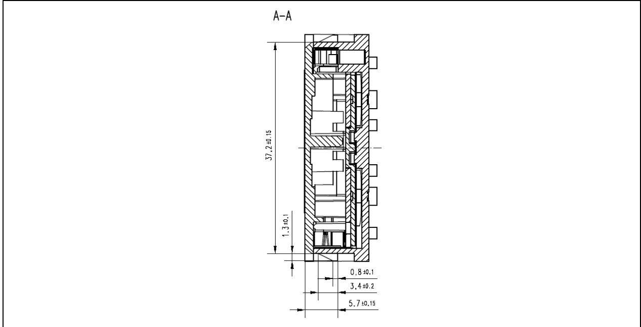
Figure 4: PTM 200C without antenna, cut A
