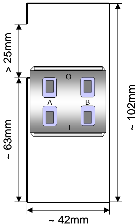
Figure 13: Laying the antenna
