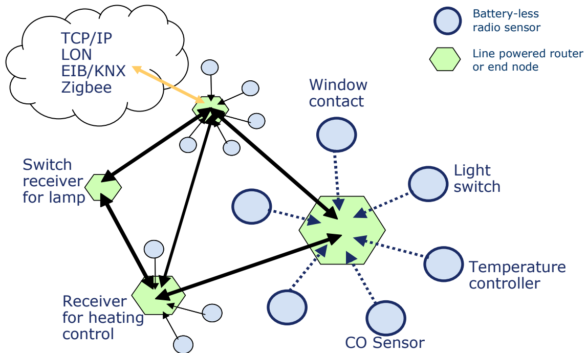
Figure 1: Example of EnOcean Wireless Networking System with battery-less nodes
