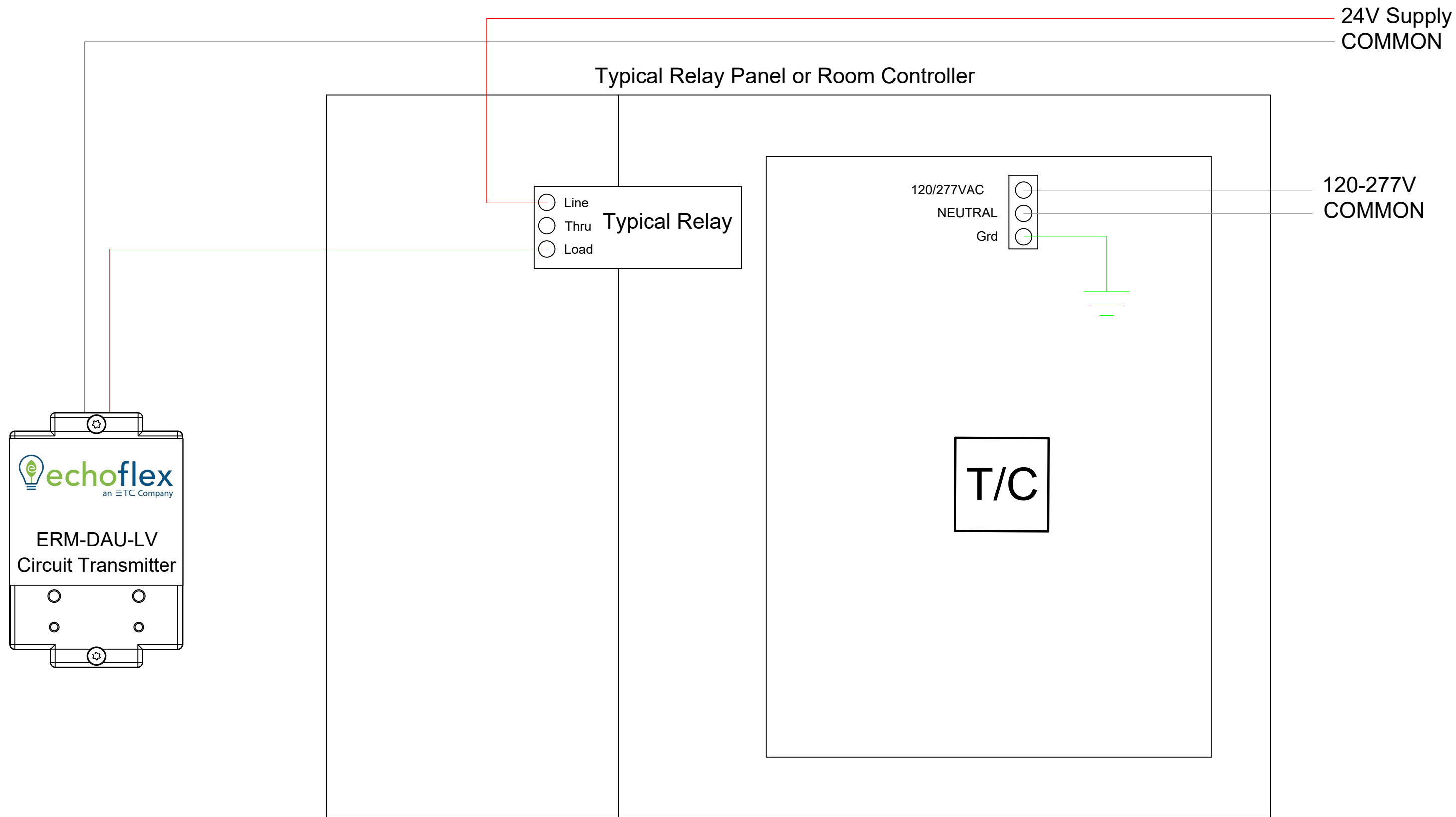
Typical Wiring Diagram - Low Voltage ERM-DAU Set as Occupancy Transmitter for Time Clock override of local occupancy control
